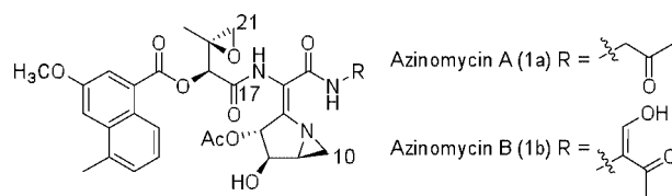
Figure 1. Structure of azinomycins A and B.
