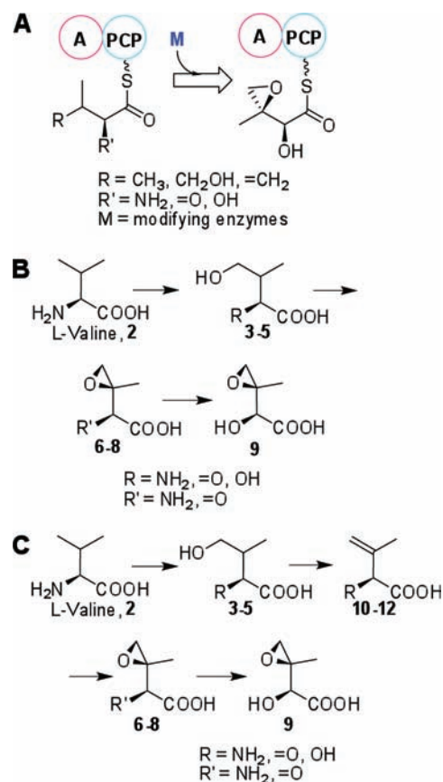
Figure 2. Possible biosynthetic routes to the epoxide moiety in the azinomycins.
