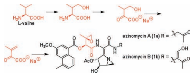
Figure 3. Biosynthetic route to the epoxide moiety in the azinomycins where failure to incorporate 11 suggests that 3-methyl-2-oxobutenoic acid 12 is epoxidized to 8 which is then reduced to 9 .
